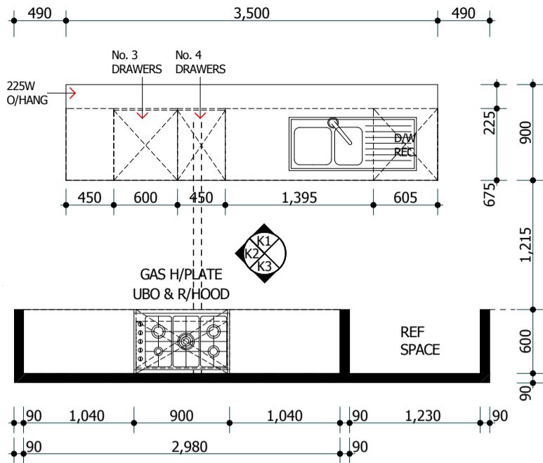
Kitchen Layout
